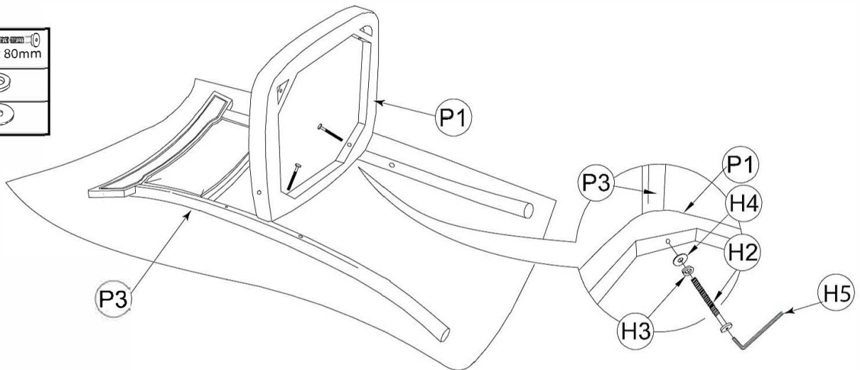
COMPLETE ASSEMBLY
