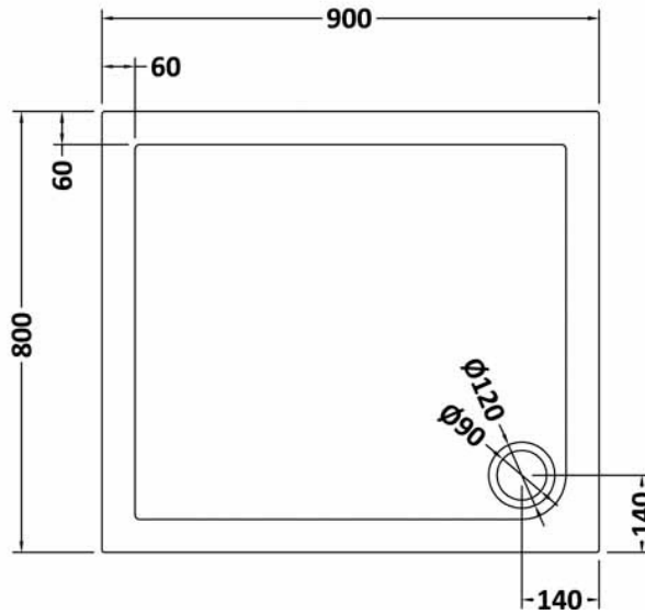
900 x 800 RECTANGULAR TRAY
