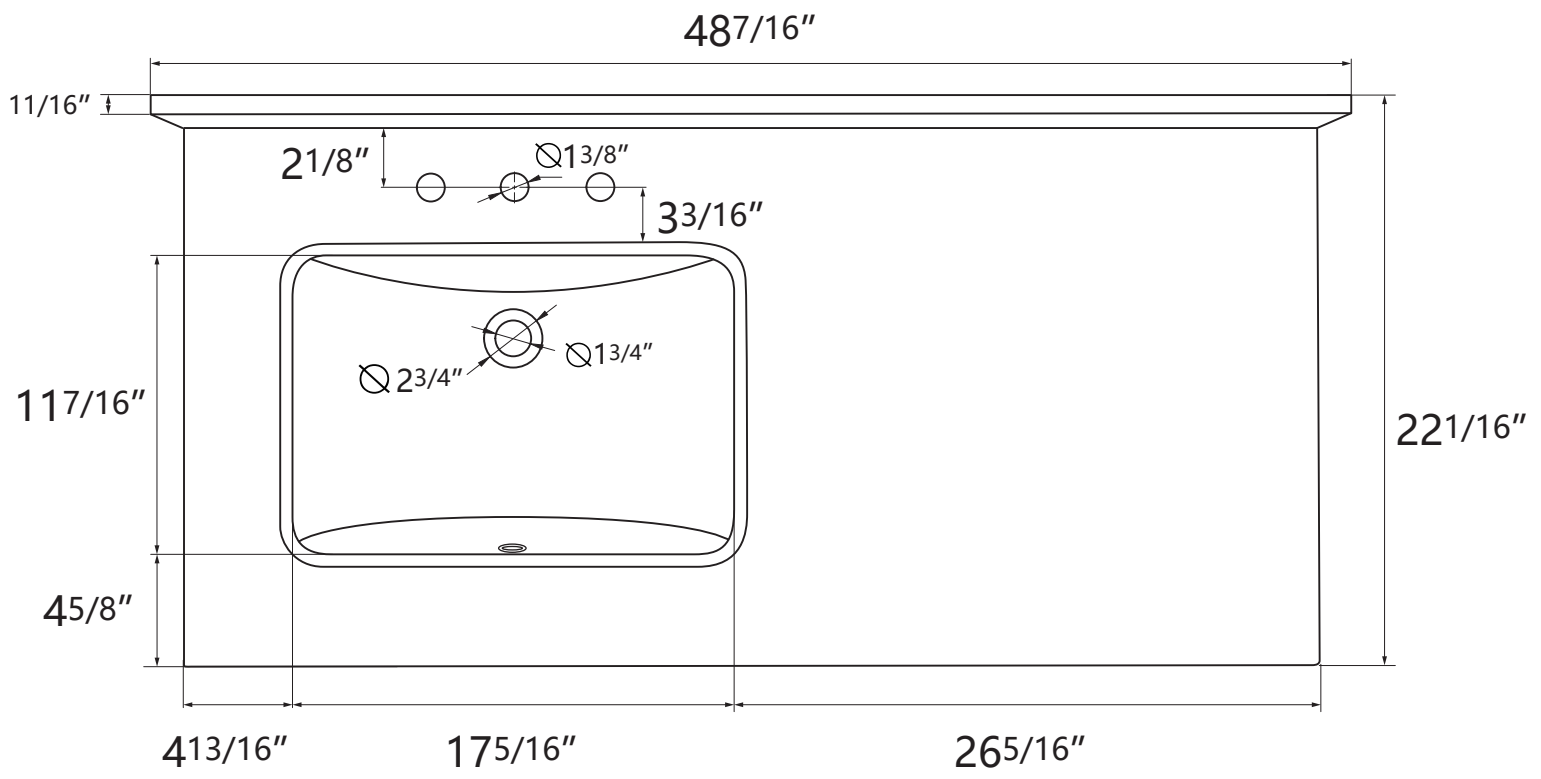
Top View
