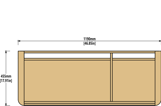
Top view of the cabinet body
