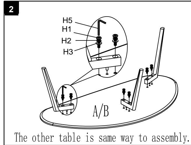
Step 2 Attach leg-L(C) leg-S(D) to panel-1(A) panel-2(B) using Allen bolt (H1) Spring washer (H2) and flat washer (H3), Tighten with allen key (H5) Stand table upright. Assembly is complete.
