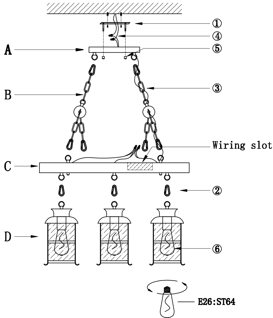
Installation sequence diagram
