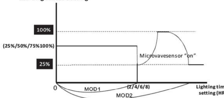
Fig-4 IPM Illumination Profile
