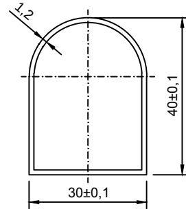
PROFILE DETAIL
