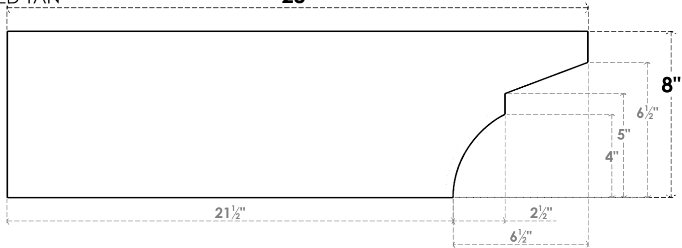
SIDE PROFILE
