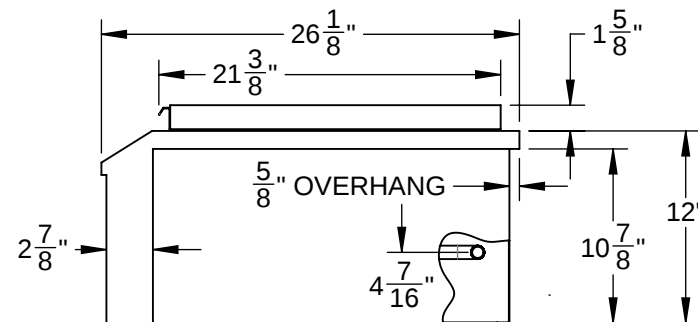
RIGHT VIEW
