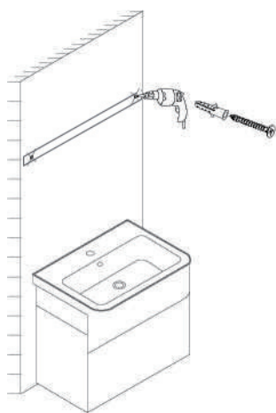
4. Secure the aluminum hanging bar with screws
