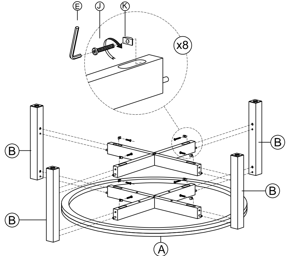
Step 2: Attach four legs and stretchers to table top
