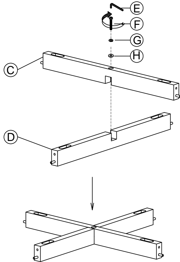
Step 1: Connect the Stretcher together
