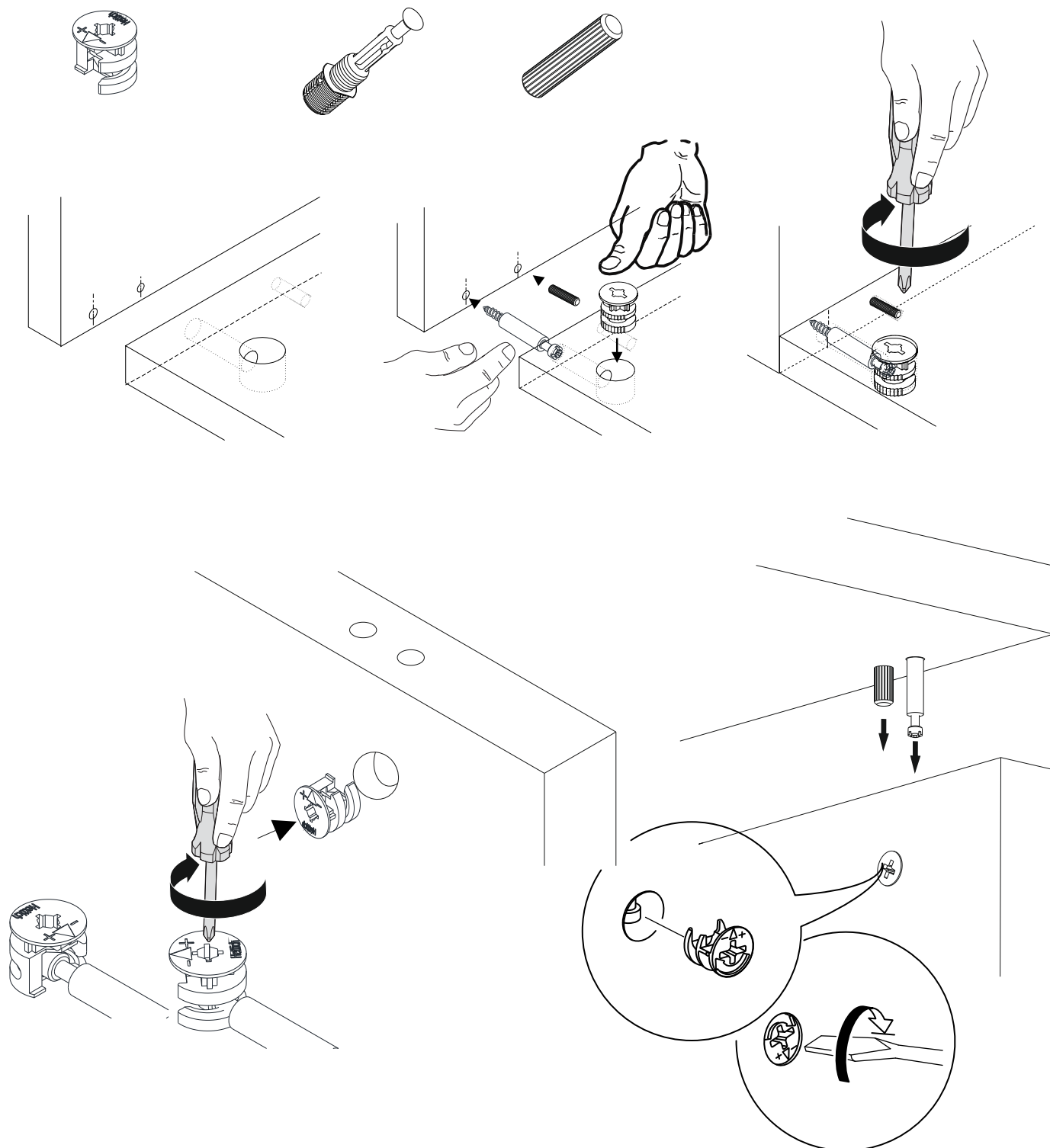
MINIFIX BODY
