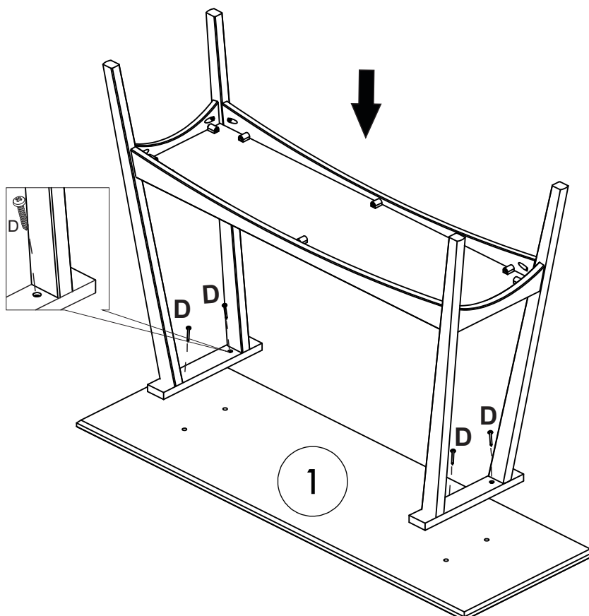
D - 4,0 x 25 Screw Qty. 4
