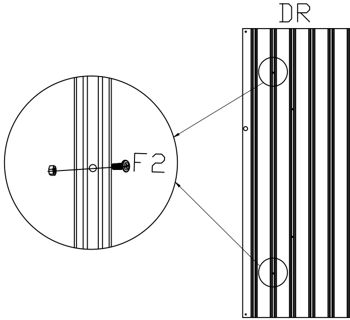
Right door panel assembly
