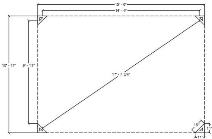
PLAN A LA BASE DES PATTES PLAN AT THE BASE OF THE LEGS
