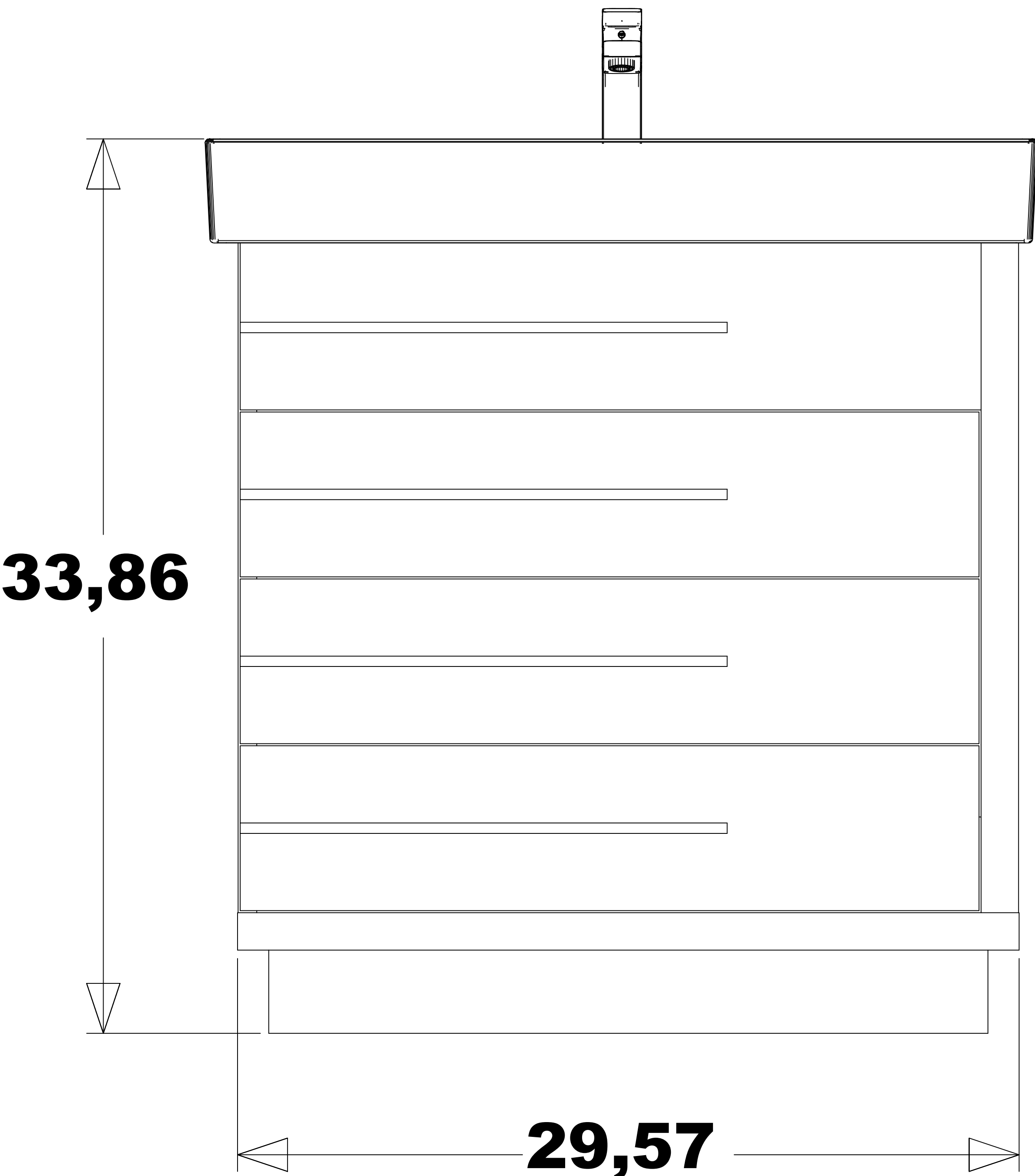
FRONT VIEW
