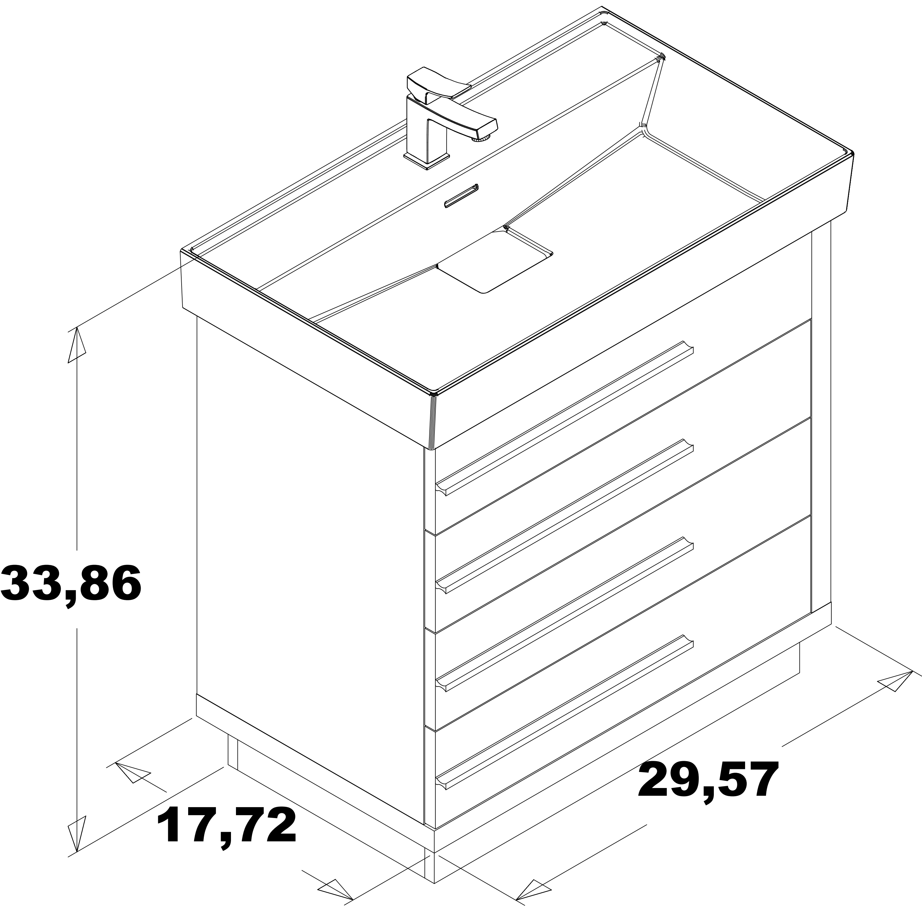
ISOMETRIC VIEW
