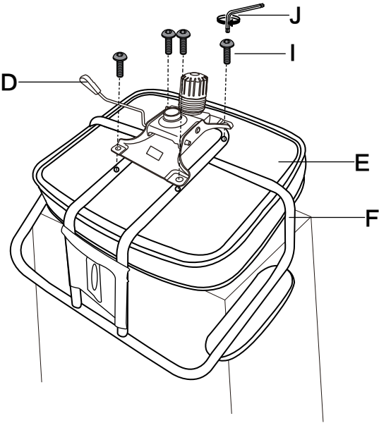
INSTALL THE FRAME AND MECHANISM ON THE SEAT CUSHION
