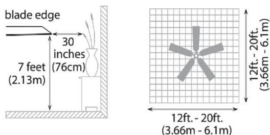
downrod installation
