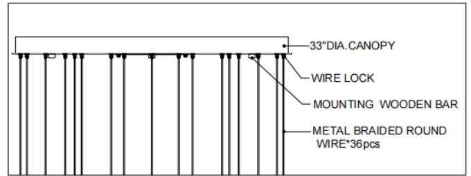
CANOPY DETAIL
