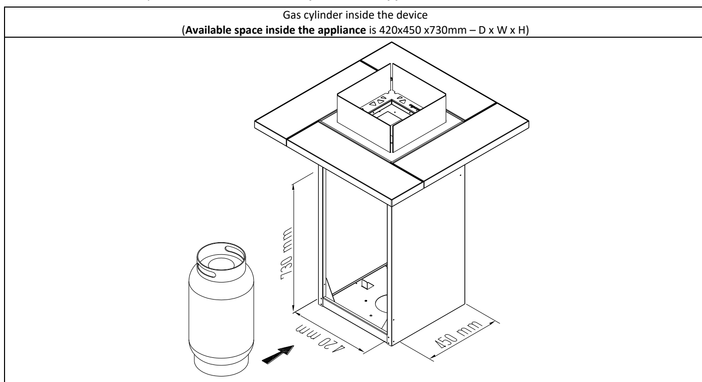
Fig. 4 –Gas cylinder space
