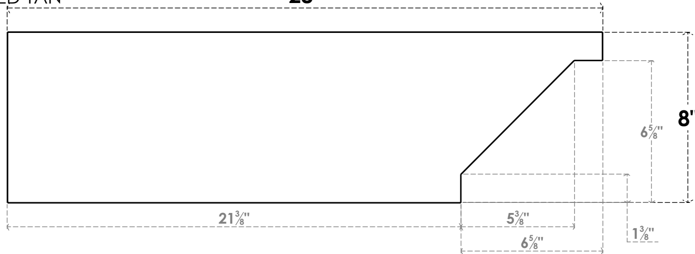
SIDE PROFILE
