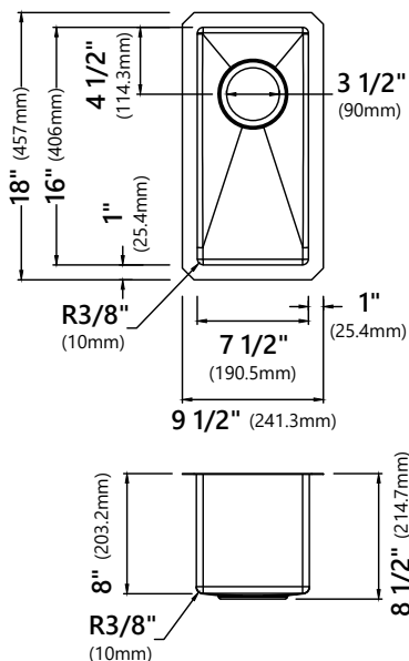
KHU101-10 9 1/2" x 18" x 8" Min Cabinet Size: 12" Drain Cap #: STC-2 Drain Model #: ST-1
