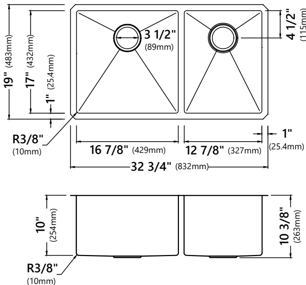
KHU103-33 32 3/4" x 19" x 10" Min Cabinet Size: 36" Matching Grid: KBG-103-33-1 and KBG-103-33-2 Drain Model #: BST-1 & ST-1
