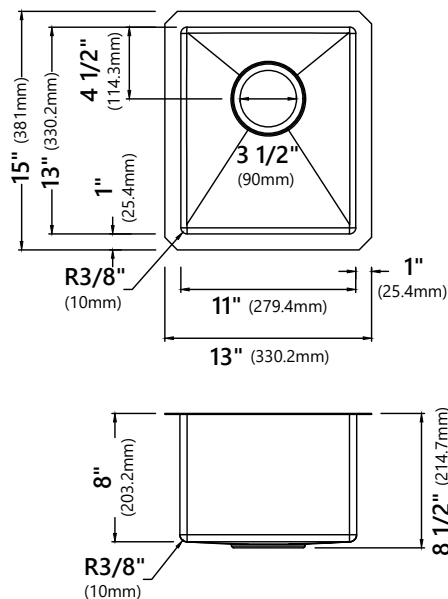
KHU101-13 13" x 15" x 8" Min Cabinet Size: 15" Drain Cap #: STC-2 Drain Model #: ST-1
