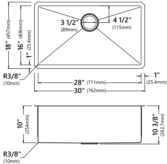
KHU100-30 30" x 18" x 10" Min Cabinet Size: 33" Matching Grid: KBG-100-30 Drain Model #: BST-1
