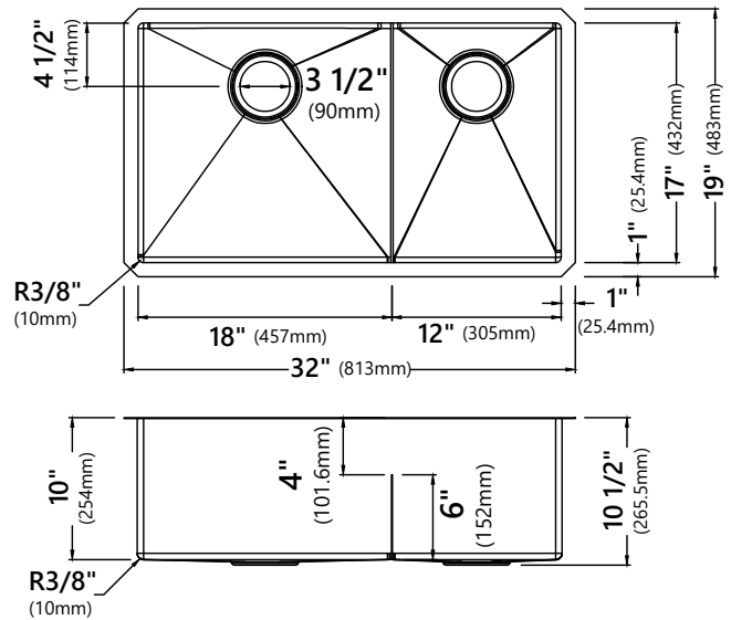
KHU103-32 32" x 19" x 10" Min Cabinet Size: 36" Matching Grid: KBG-103-32-1 and KBG-103-32-2 Drain Model #: ST-1 x 2 Drain Cap #: STC-2 x 2
