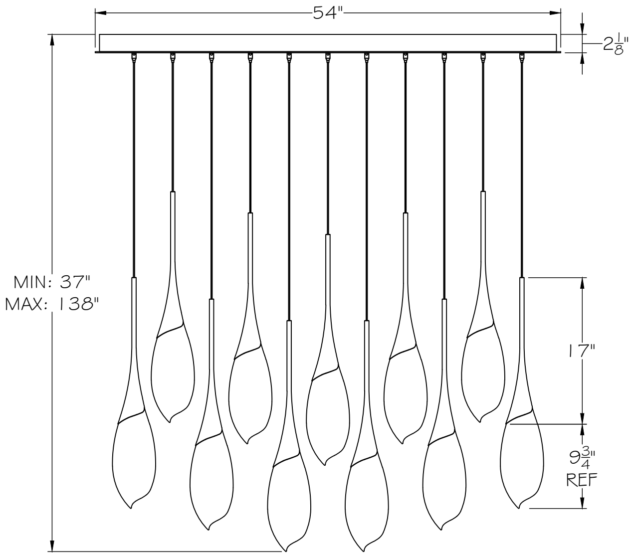
FRONT VIEW
