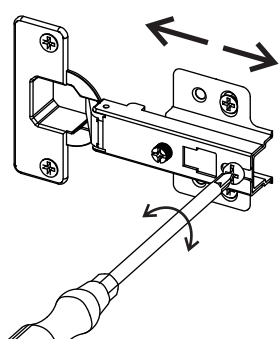
Depth adjustment
