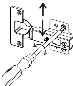
Height adjustment
