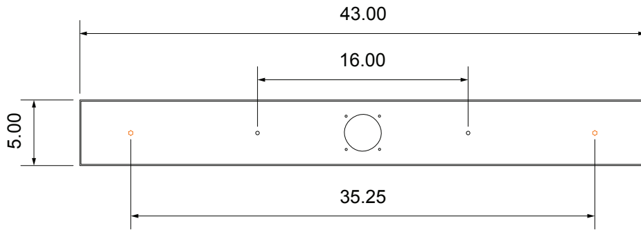
Top View - Mounting Plate
