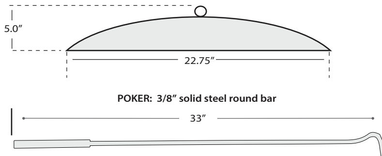
SPARK SCREEN: Black Painted 0.28 8-mesh steel screen 3/8" solid steel round bar frame construction
