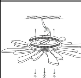
⑧ Screwing the ceiling light to the mounting platte.
