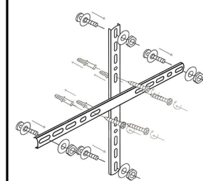
③ Filling the hole with plugs and fixing the mounting plate by screws
