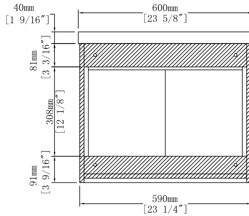
Back View
