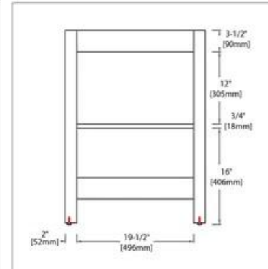
VANITY BACK
