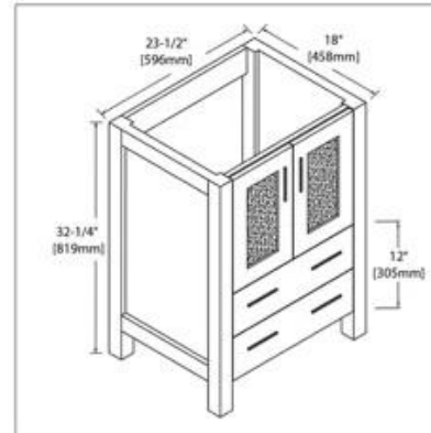
VANITY FRONT
