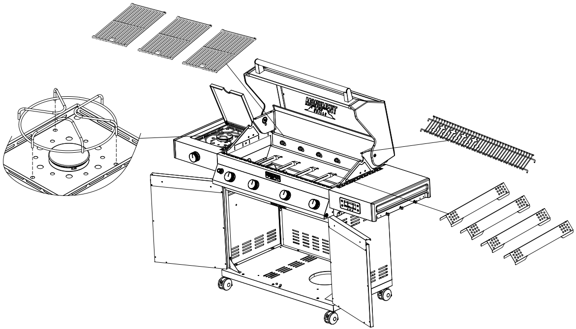
Put Cooking Grid, Warming Rack ,Pan Bracket and Flame Tamer into the relevant place. Figure 19
