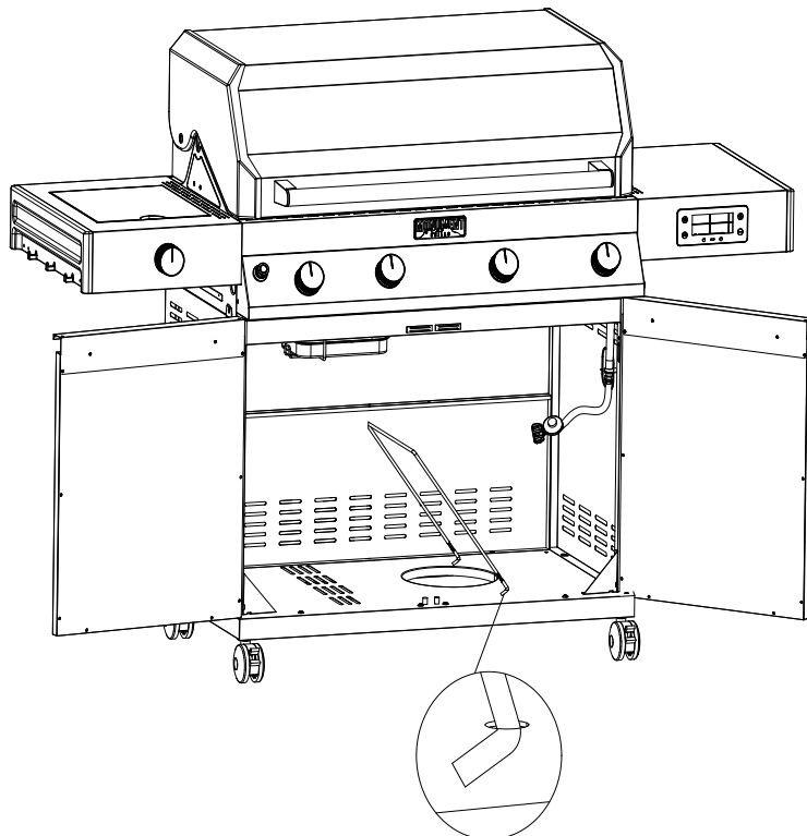
Install Gas Tank Holding Line onto the bottom plate. Figure 20
