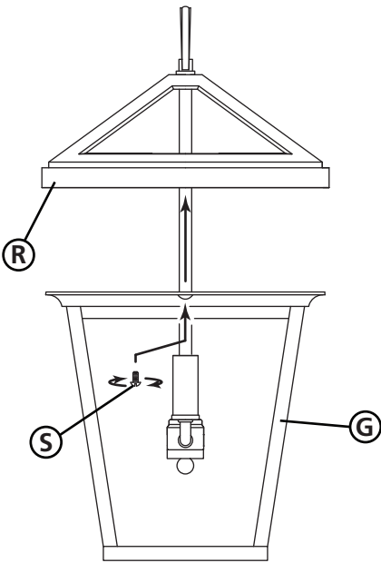
DRAWING 2 - ASSEMBLY
