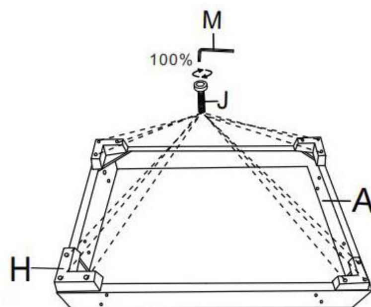
Seat frame 3
