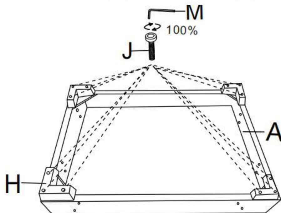
Seat frame 4
