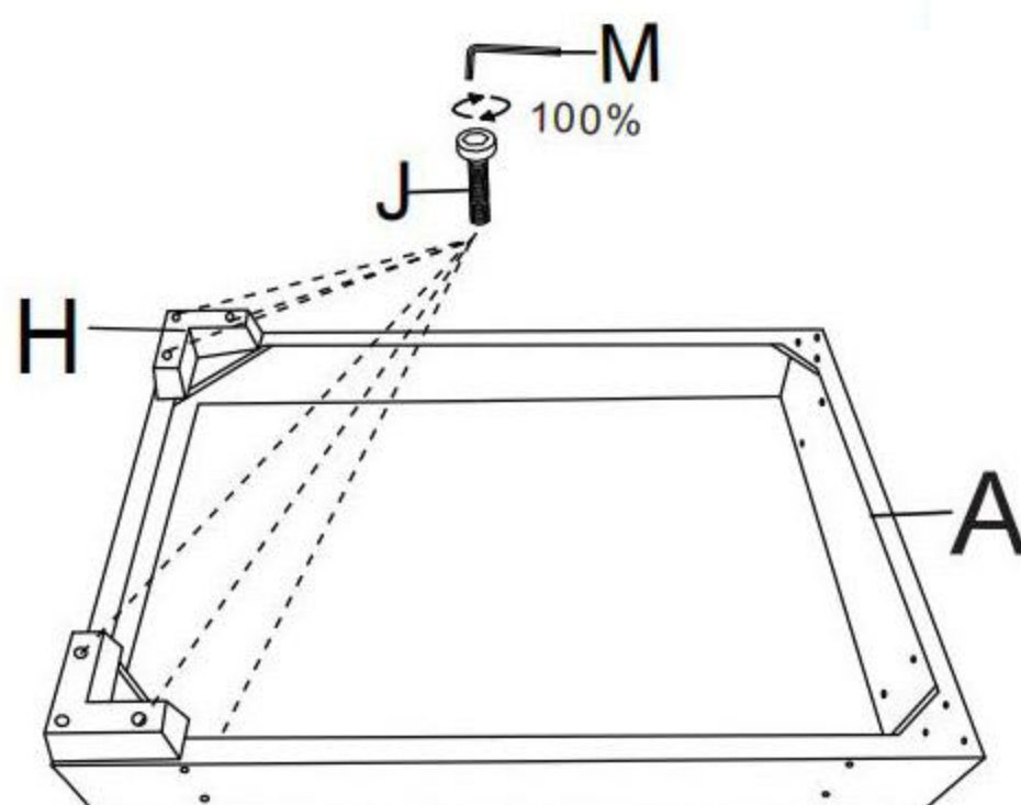
Seat frame 2
