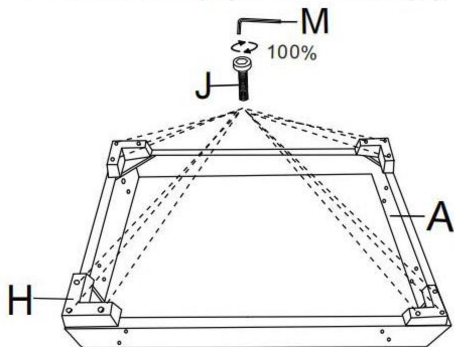
Seat frame 3
