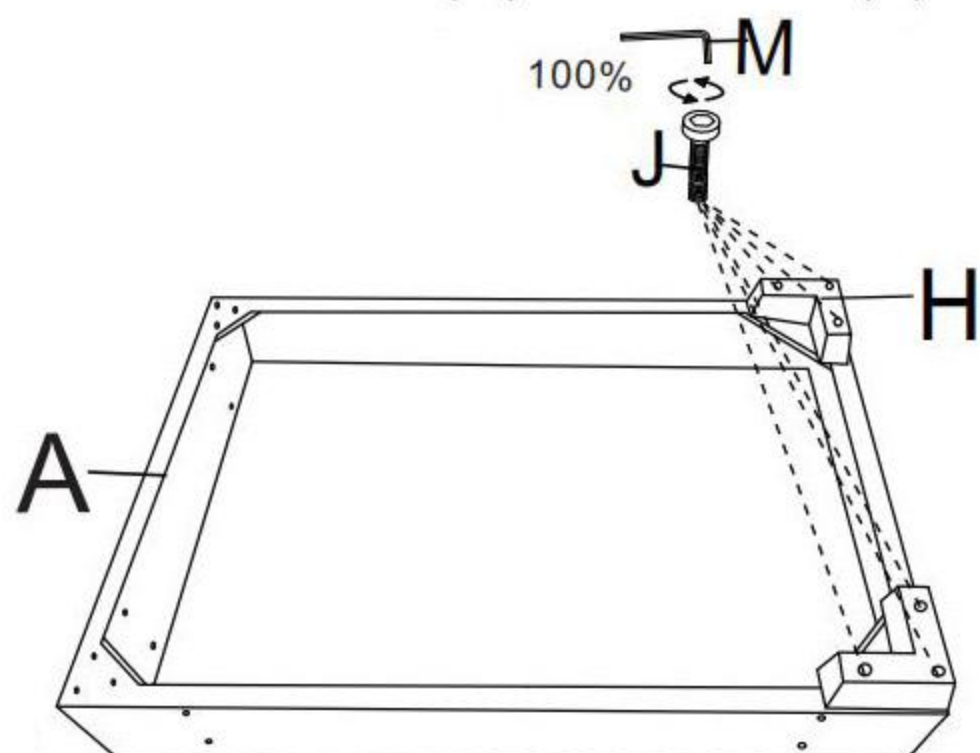
Seat frame 1
