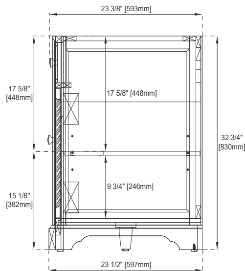
Side View 2
