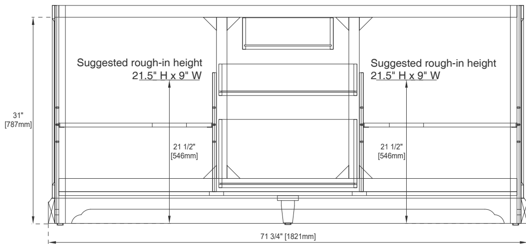
Back View
