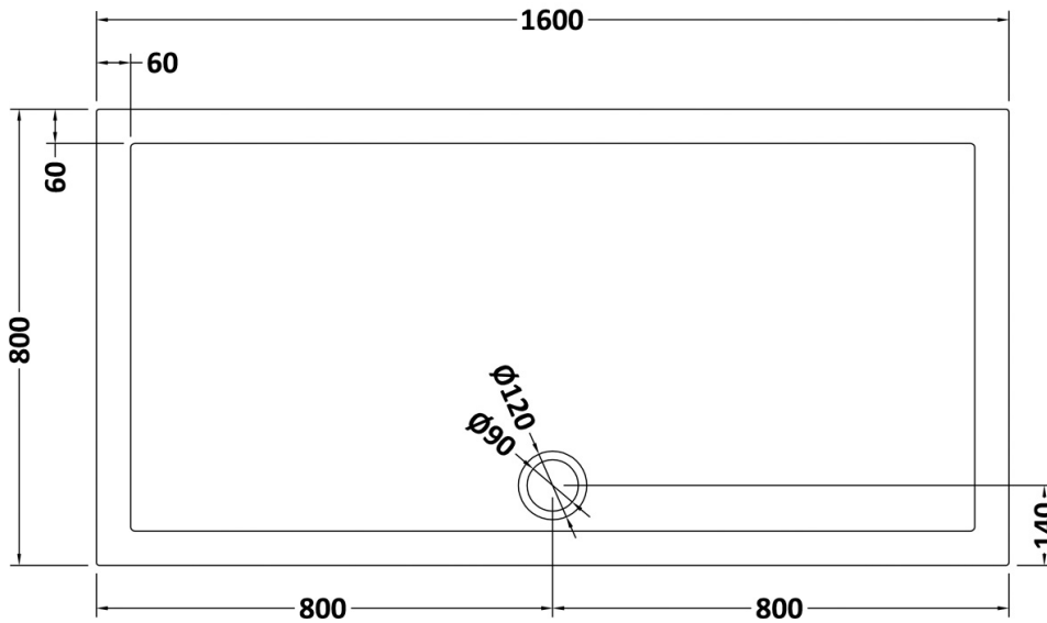
1600 x 800 RECTANGULAR TRAY
