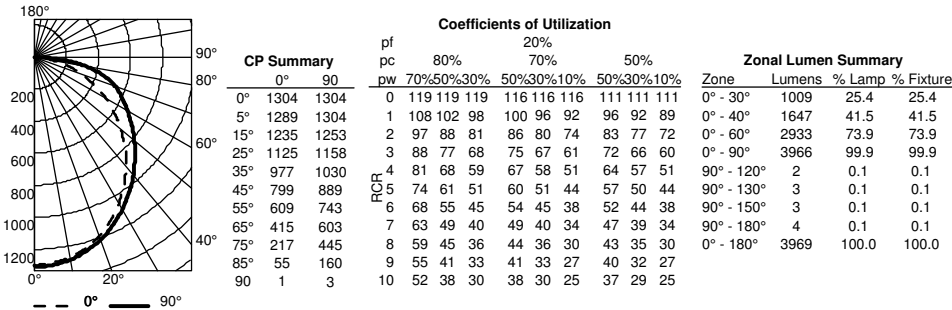
BLC 2X2 40L LP835, 3970 Delivered Lumens, tested in accordance to IESNA LM-79.
