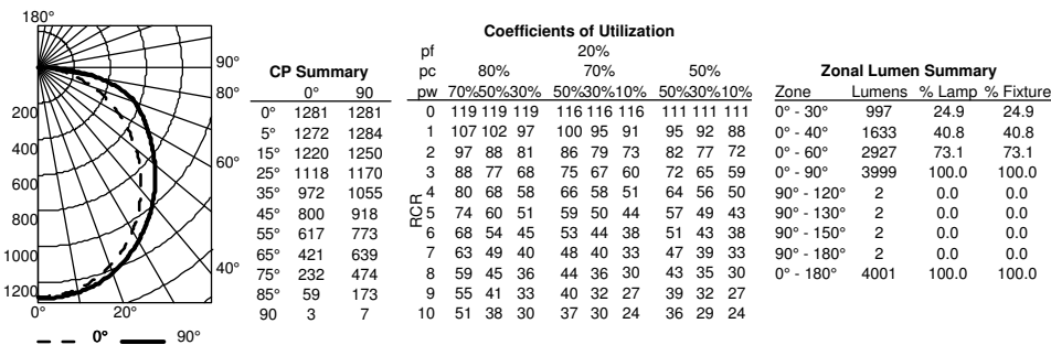
BLC 2X4 40L LP835, 4003 Delivered Lumens, tested in accordance to IESNA LM-79.
