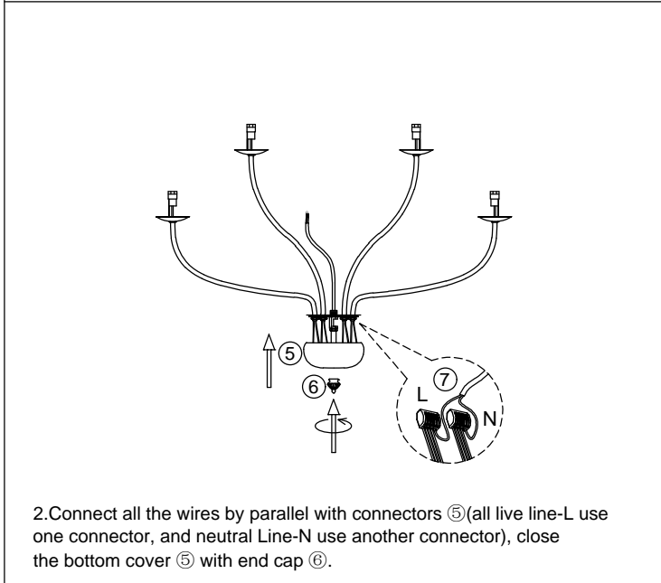
2. Connect all the wires by parallel with connectors ⑤ (all live line-L use one connector, and neutral Line-N use another connector), close the bottom cover ⑤ with end cap ⑥. 3. Let the wire go through the hanging tube ⑧ and ⑨, rotate to install to the fixture.
