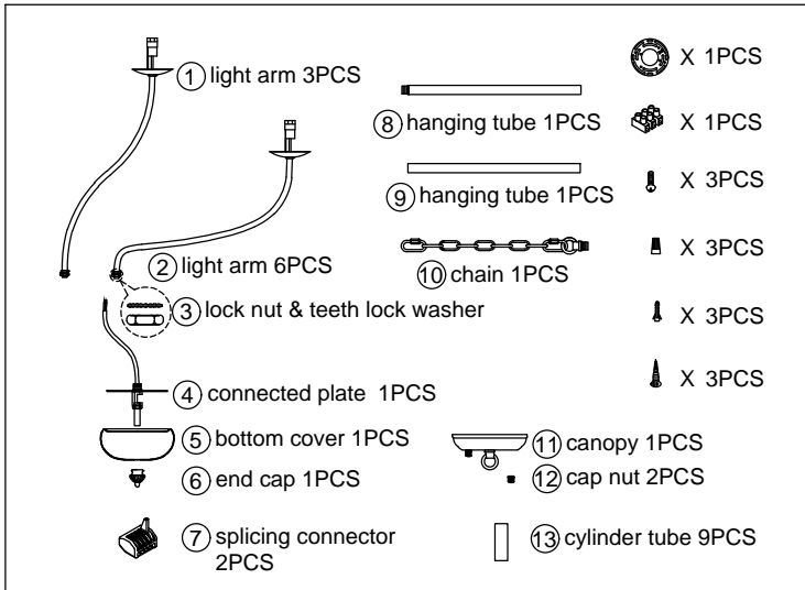
1. Install the light arms on the connected plate ④ with lock nut & teeth lock washer ③.
