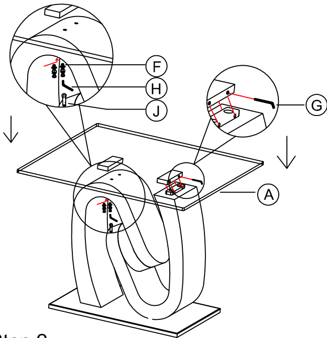
Step 2 Put the glass top on the pedestal and screw the glass top to pedestal
