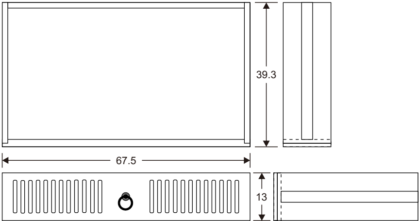
DRAWER DETAIL
