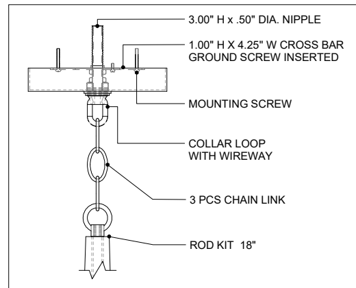
CANOPY DETAIL
