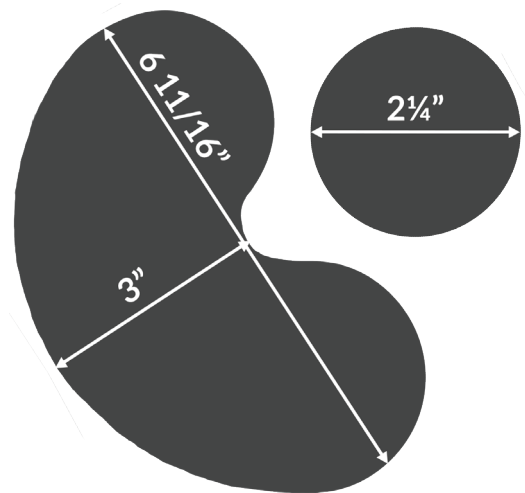
INTAKE MEASUREMENTS
