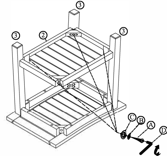
ASSEMBLY - SHELF TO LEGS AS SHOWN
