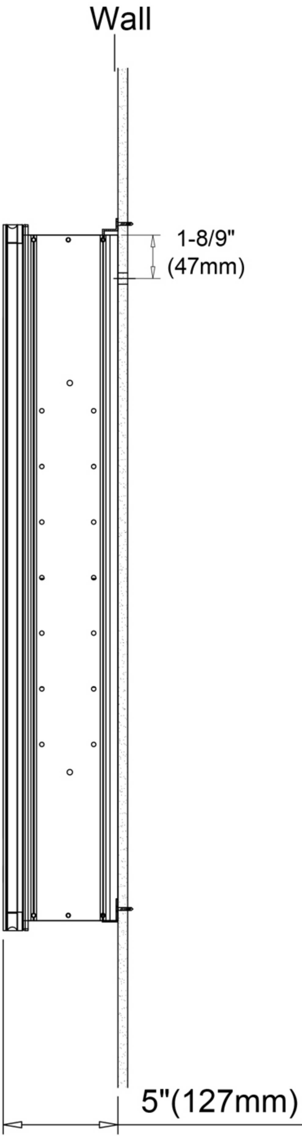
Surface Mount
