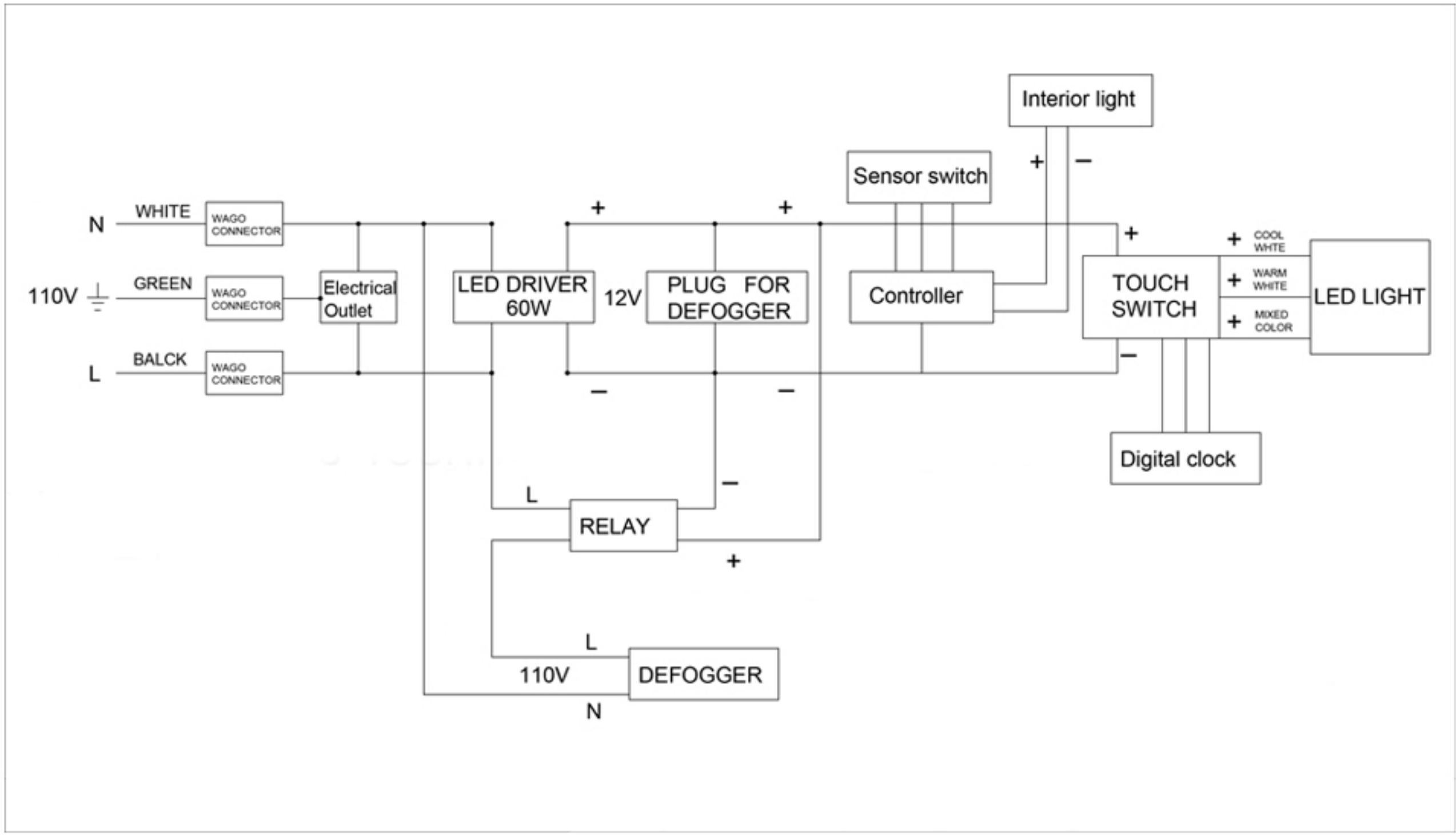
Circuit Diagram
