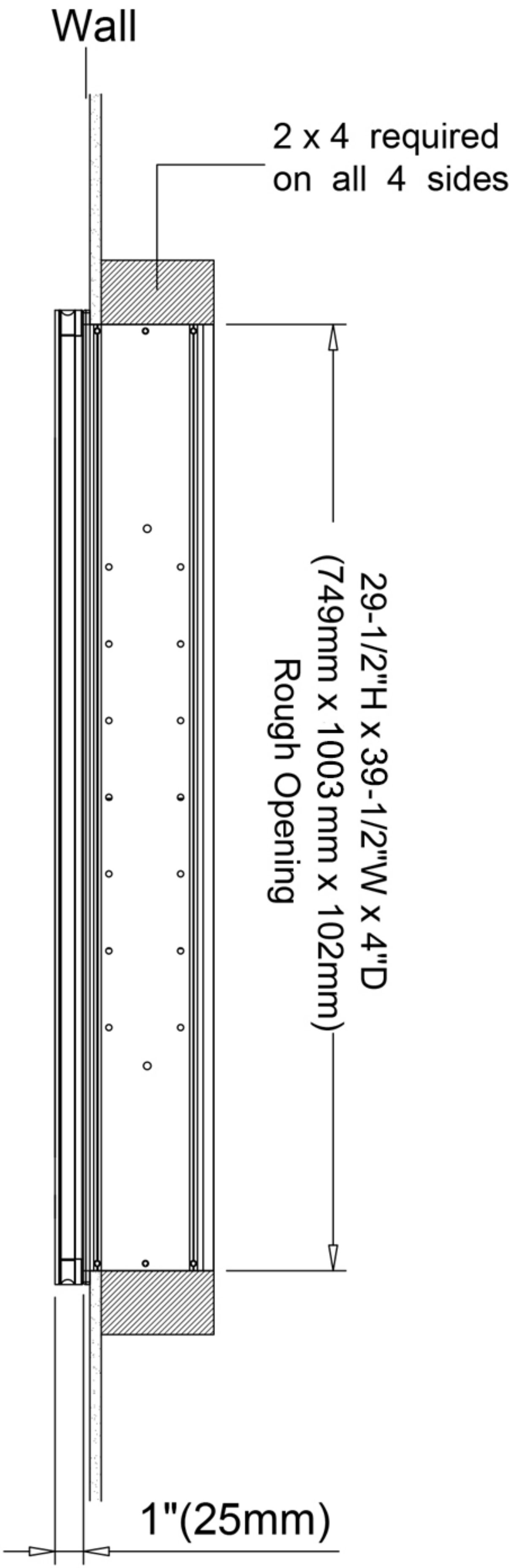
Recessed Mount
