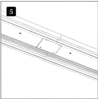
5 Join the two track sections together using the connector
