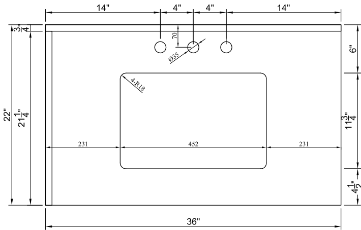
TOP VIEW OF VANITY CABINET
