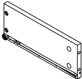
LEFT DRAWER SIDE QTY 2
