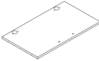
Door Panel (Left) - 2pcs
