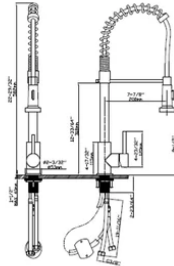
CRITICAL DIMENSIONS
