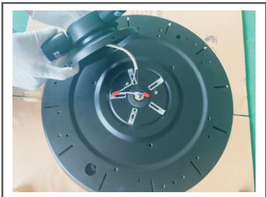
Step 2. Connect the power cable
