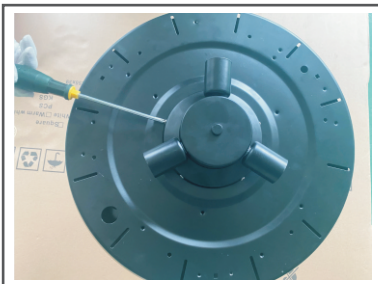
Step 3. Fix the lamp holder with screws
