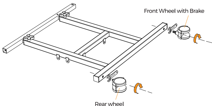
Front Wheel with Brake
